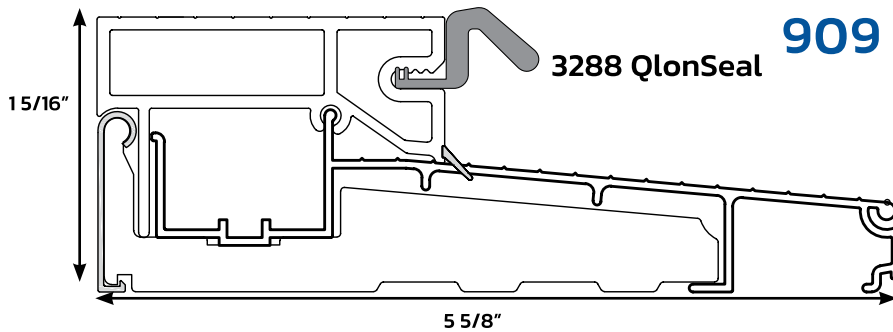
909 Composite Outswing Sills
