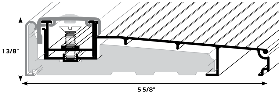
901 Composite Inswing Sills
